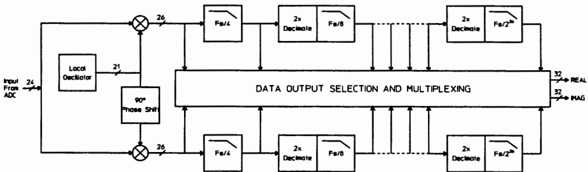
Zoom and Decimation Filtering - Block Diagram
